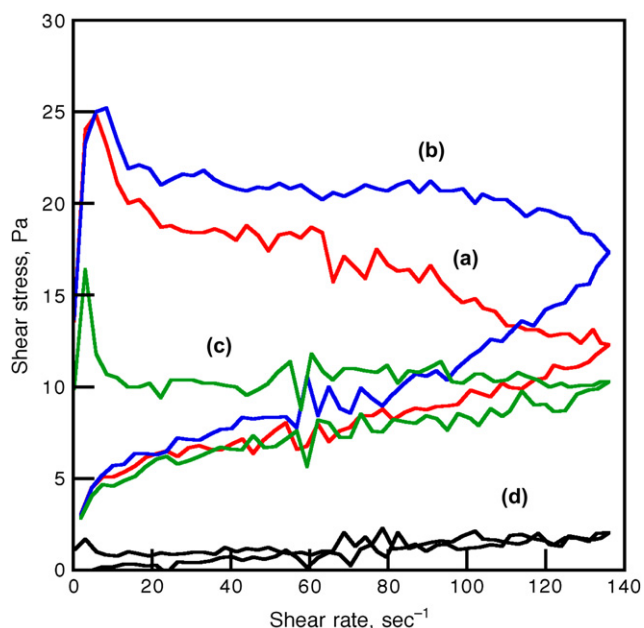
Fig. 2. Viscosity curves of the DNFB-PR2000 solution in DMSO at 5 wt% concentration (a–c) and the DNFB-PR3350 solution in DMSO at 5 wt% concentration (d). (a) First measurement, (b) second measurement performed 1 h after the first measurement, (c) third measurement performed just after the second measurement and (d) first measurement after leaving 1 h in a rheometer.
